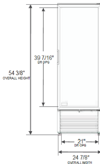
ELEVATION VIEW
