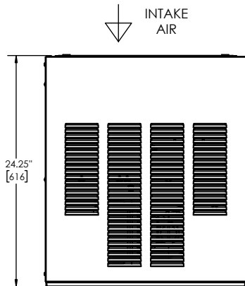
PLAN / TOP VIEW
