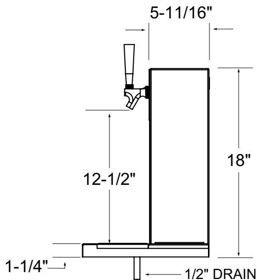
SIDE ELEVATION
