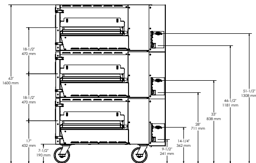
1624 Gas Triple Stack Side View
