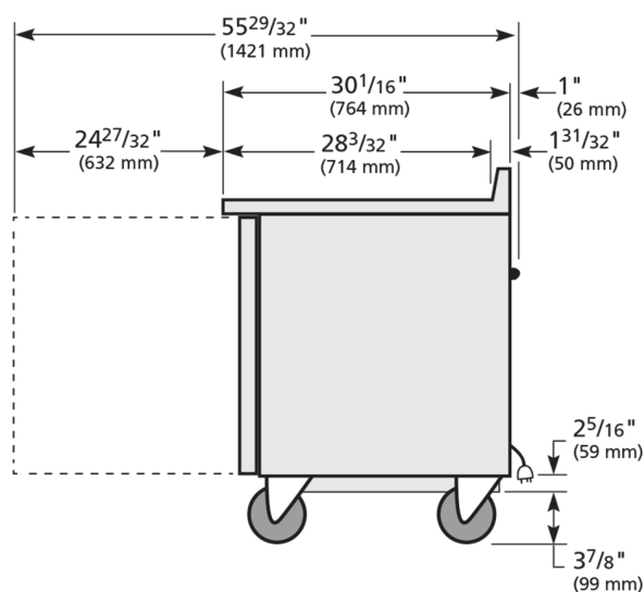
RIGHT VIEW
