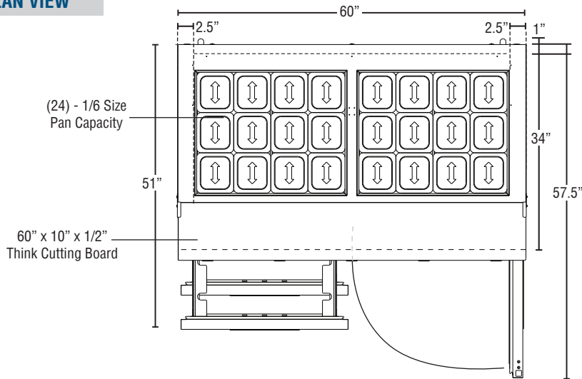
PLAN VIEW
