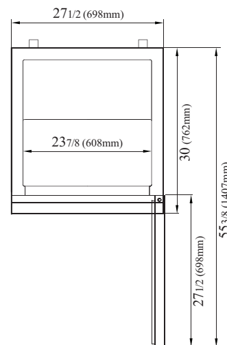
TOP VIEW
