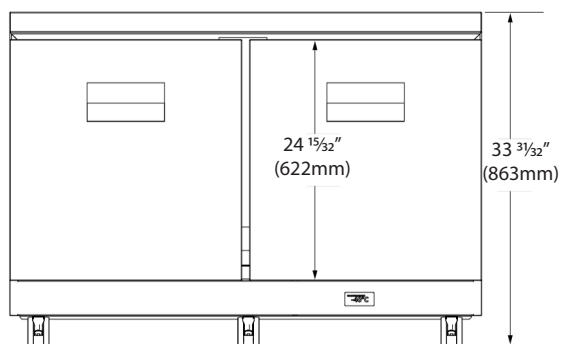
Front (UCRE336, 348, 360)
