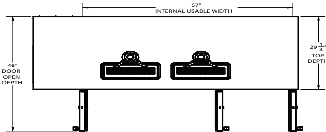
ELEVATION VIEW
