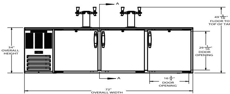
ELEVATION VIEW
