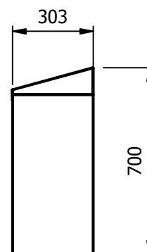
Sliding doors with sloping roof
