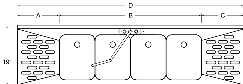
PLAN VIEW
