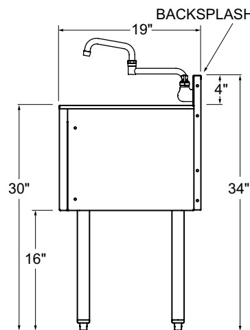
SIDE ELEVATION
