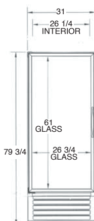
ULG30 FRONT VIEW
