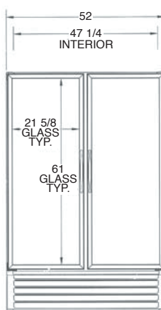
ULG50 FRONT VIEW
