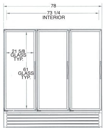
ULG80 FRONT VIEW
