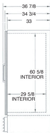
ULG30, ULG50, ULG80 SIDE VIEW
