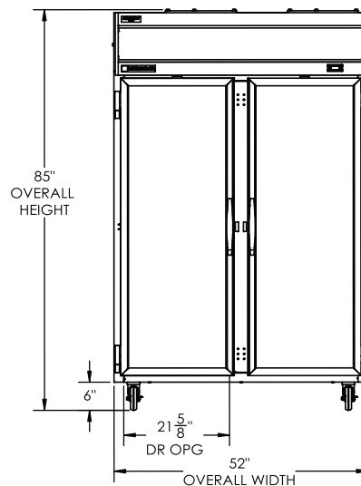
ELEVATION VIEW
