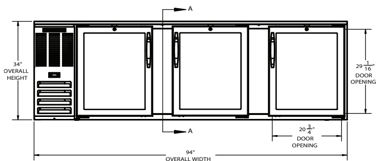
ELEVATION VIEW
