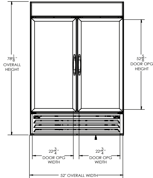
ELEVATION VIEW
