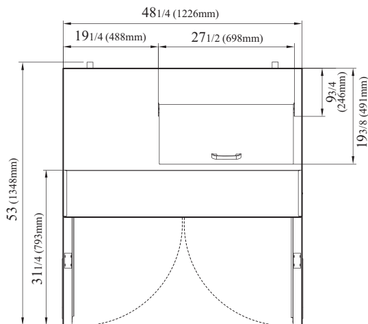
TST-48SD-08S-N-LW TOP VIEW
