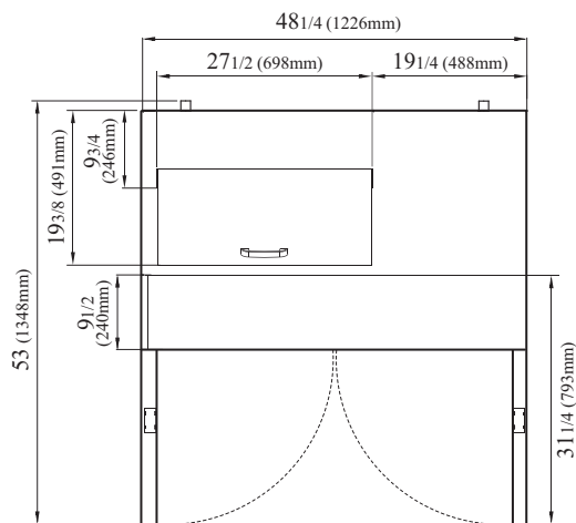
TST-48SD-08S-N TOP VIEW
