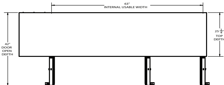
ELEVATION VIEW
