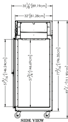
RLT332WUT-FHS
