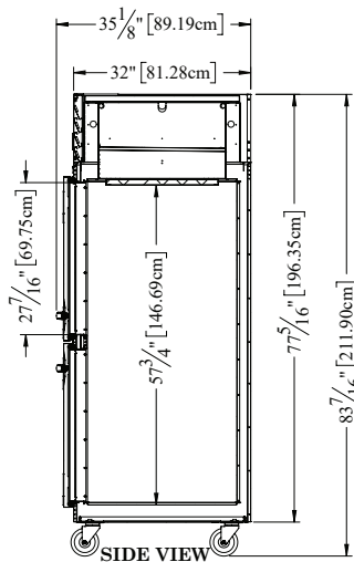
RLT332WUT-HHS
