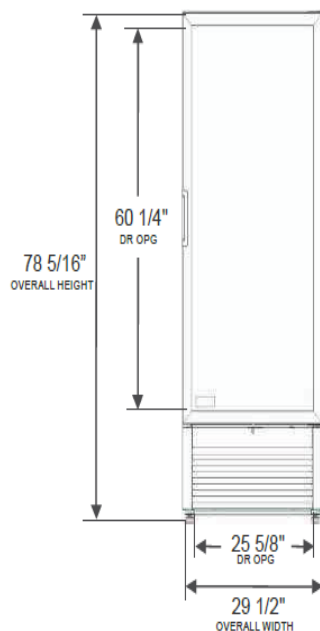
ELEVATION VIEW
