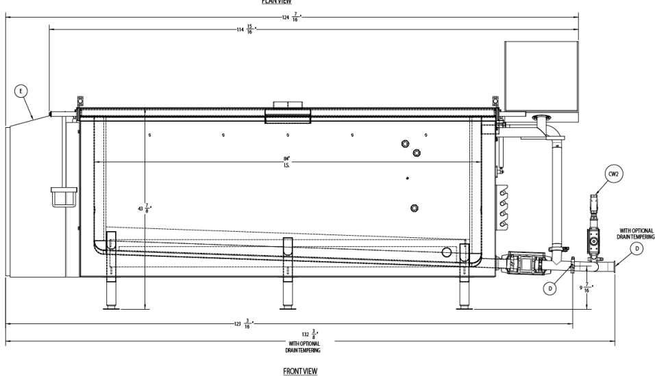
ZPCWBCC075 PRODUCT COOKER COOLER/HBCC075-60MMAN ASSY
