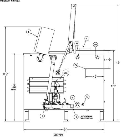
ZPCWBCC075 PRODUCT COOKER COOLER/HBCC075-60MMAN ASSY
