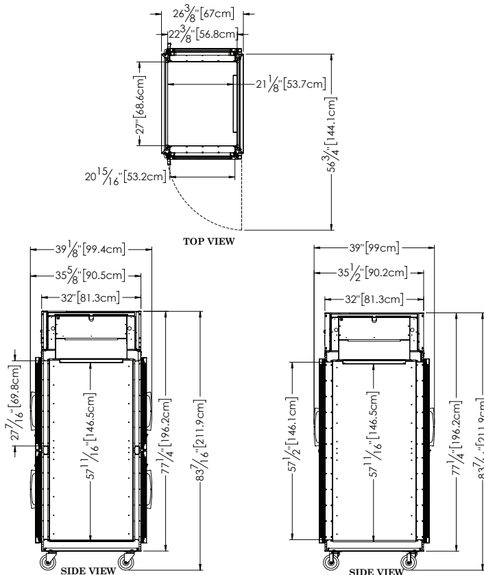
Shown on optional 6" casters
