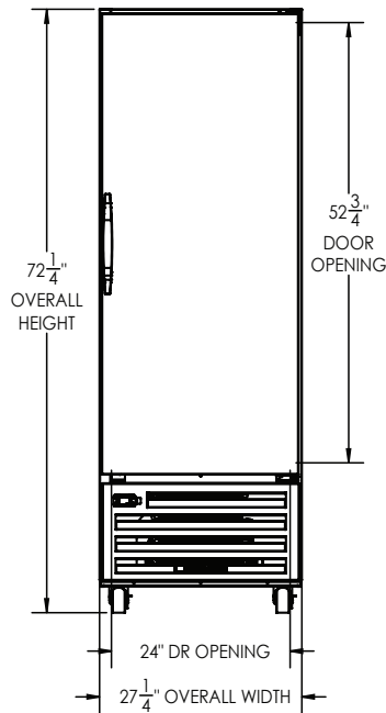
ELEVATION VIEW
