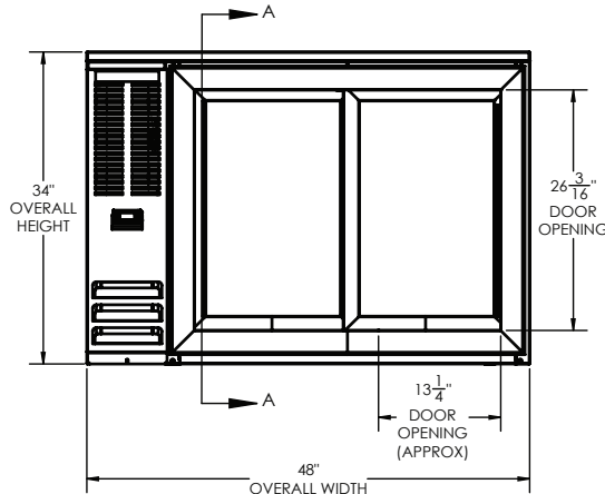
ELEVATION VIEW
