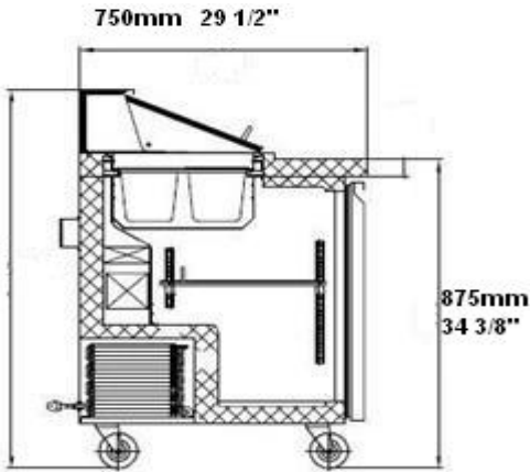
Section View
