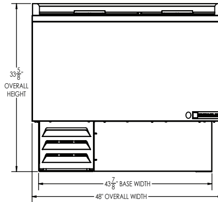
ELEVATION VIEW
