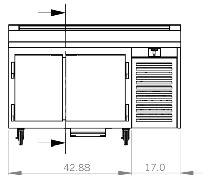
Elevation View
