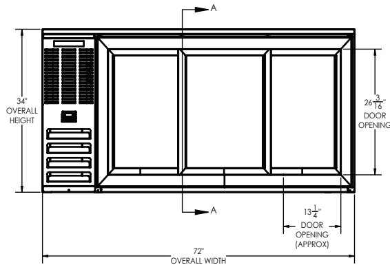
ELEVATION VIEW
