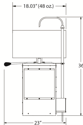
End View
