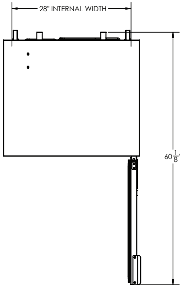
PLAN VIEW
