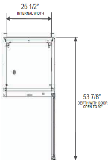
PLAN VIEW
