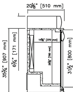
RIGHT VIEW
