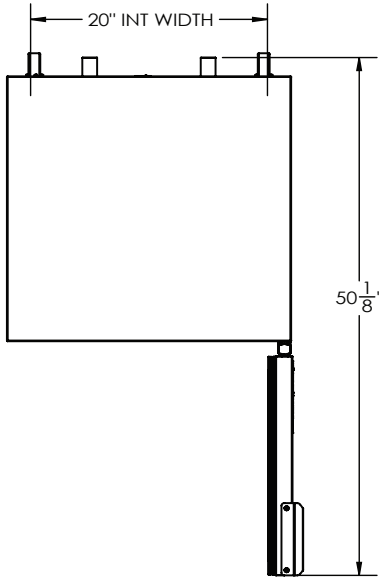
PLAN VIEW
