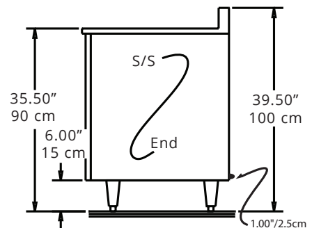
End Elevation ST4048P
