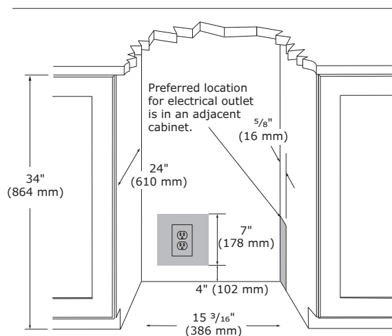
Cabinet Cut-Out
